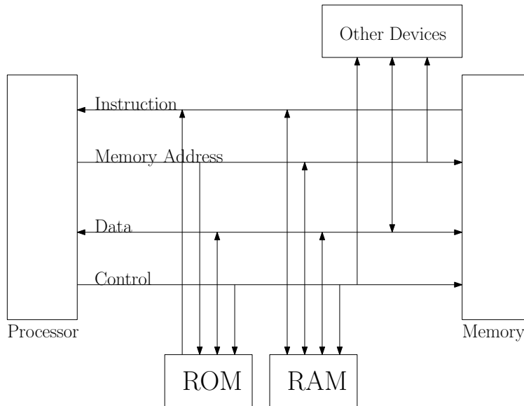
Figure 9: A simple computer architecture.
