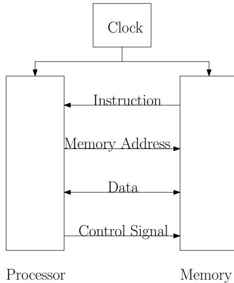
Figure 8: Types of signals transferred between a processor and a memory.
