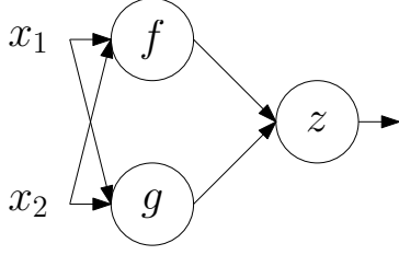
Figure 1: A network (resp. computational model) consisting of three neurons (resp. computational units). All of them are 2-input-1-output neurons.
